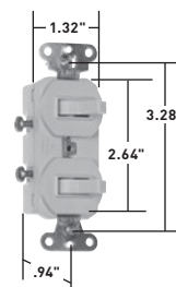
Combination Switches
